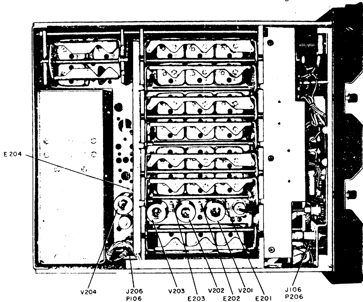
Figure 7. (Superseded) Receiver tube, plug, and test point locations, top view.
