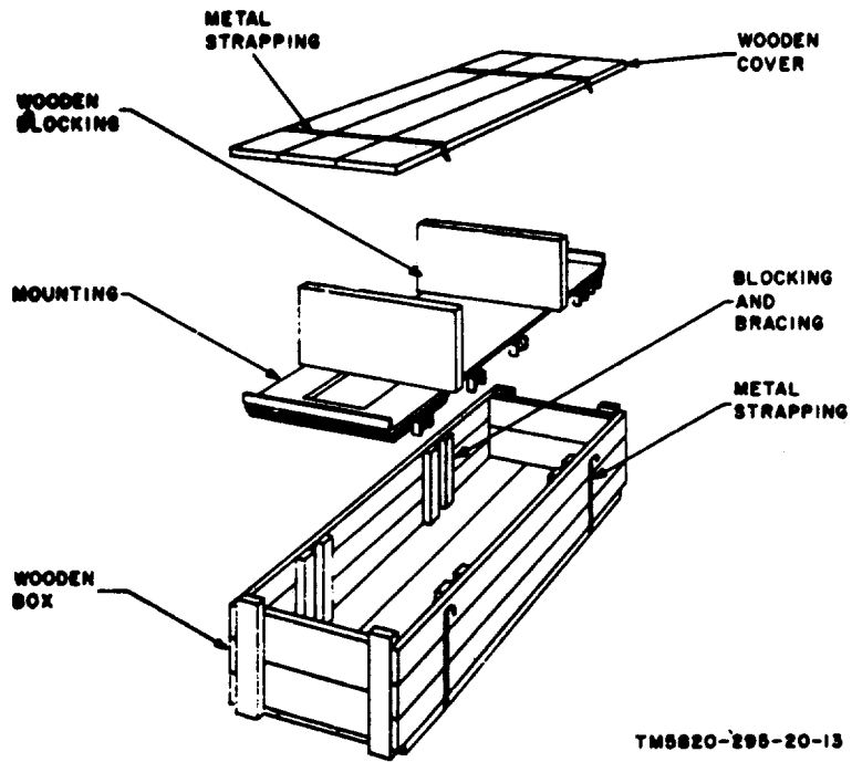
Figure 18. Mount, repackaging diagram.
