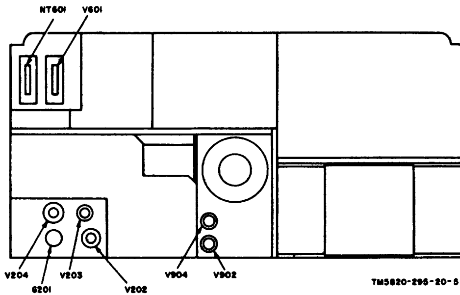
Figure 6. Transmitter tube and plug location, rear view.
