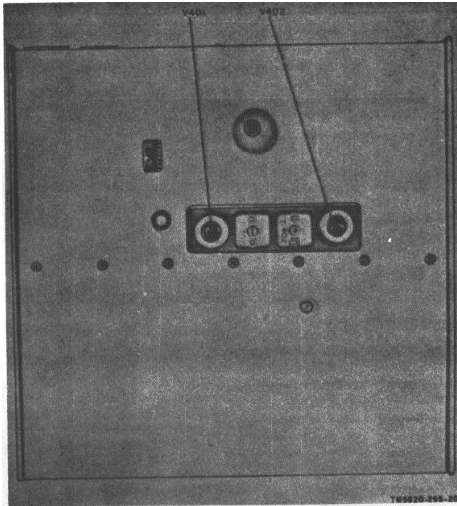
Figure 9. Receiver tube location, rear view.
