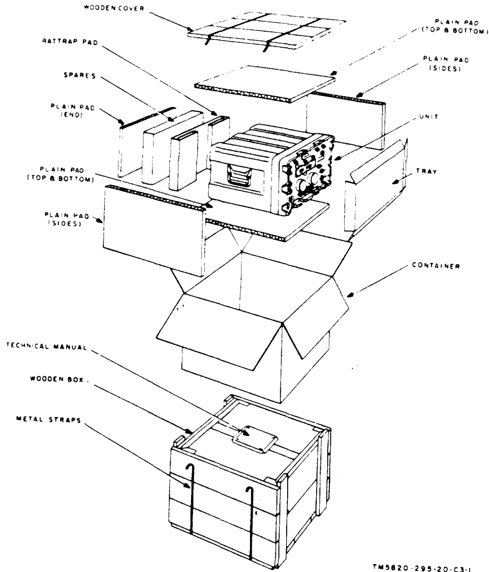
Figure 10.1. Typical packaging.
